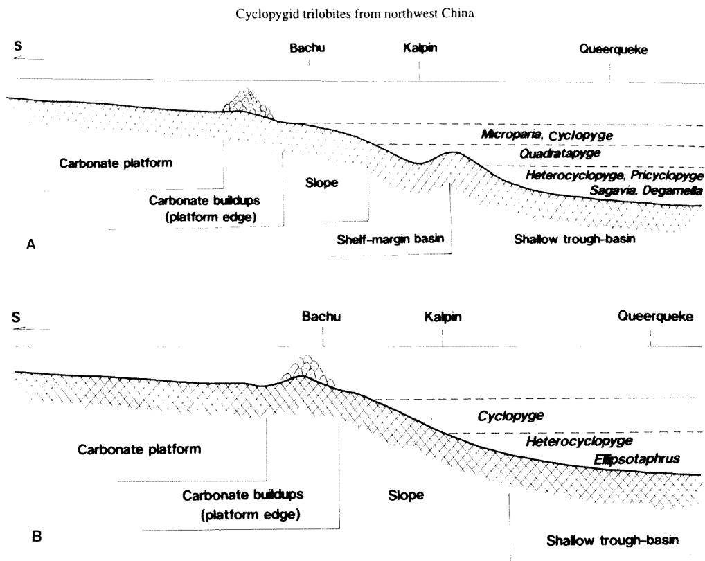
Figure 2 Palaeogeographic profiles across the Tarim Block (after Zhou et al. in Zhou and Chen 1990) showing the depth differentiation of the mesopelagic cyclopygids during the late Llandoili-earliest Caradoc (A) and early Caradoc (B).
